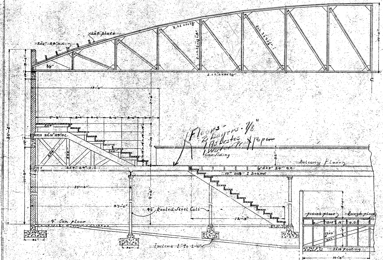
CROSS SECTION
